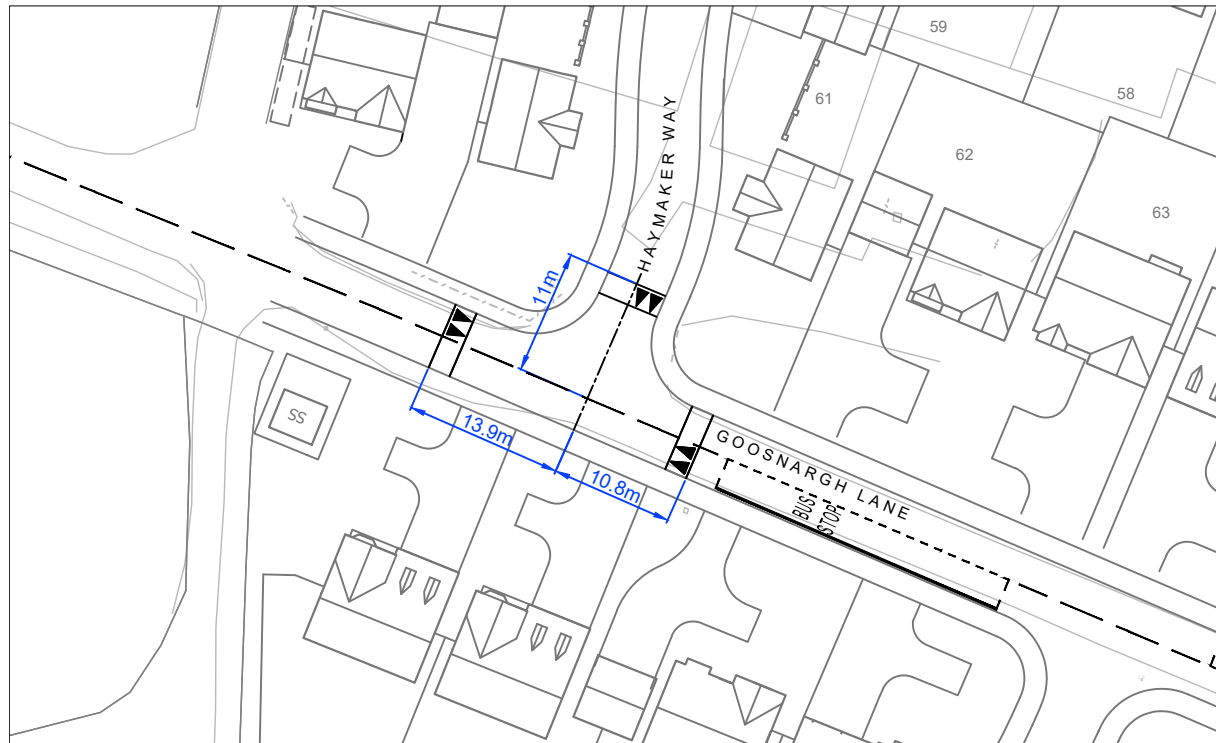
TRO PLAN - ROAD HUMPS
