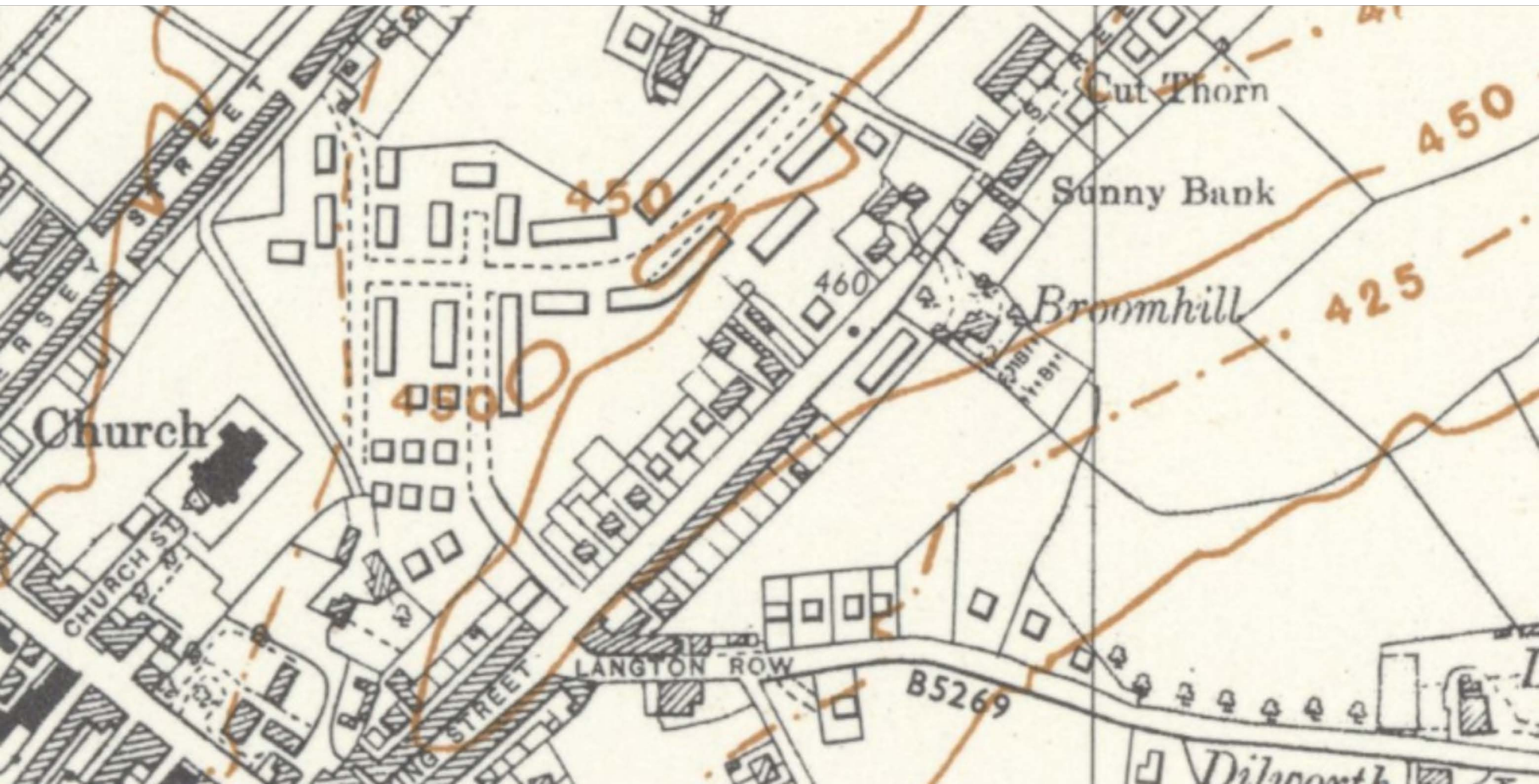
Enlarged extract of 6 inch OS Plan SD 63NW surveyed and revised 1930-1955 and published 1956
