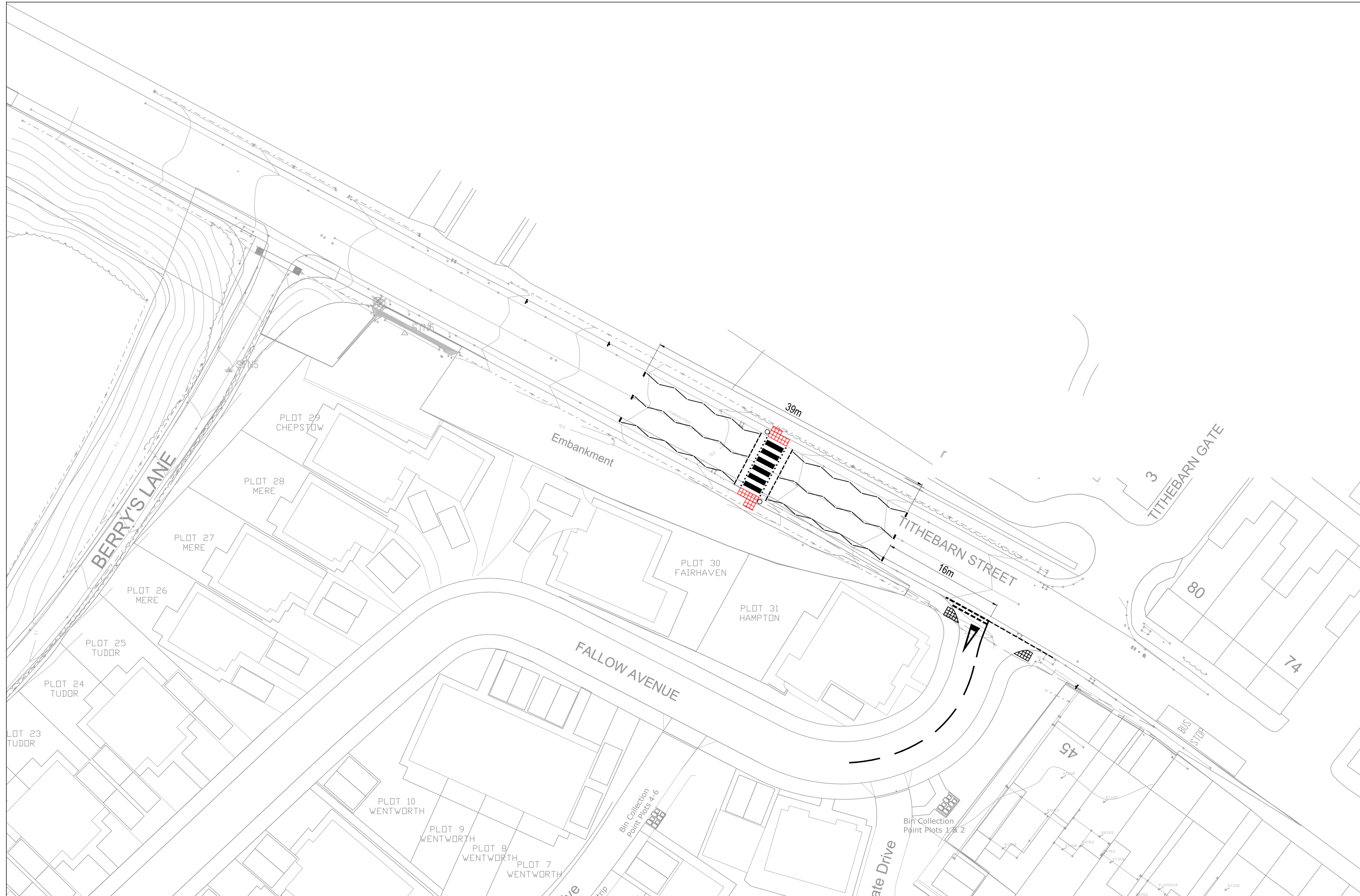
DEVELOPMENT ACCESS - PROPOSED ROAD MARKINGS AND SIGNAGE (1:250)
